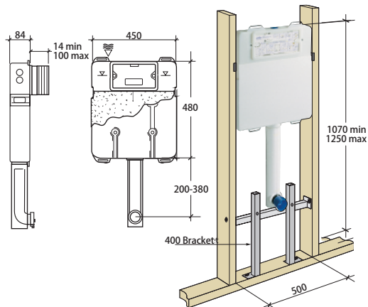
Max working pressure for all cisterns is 5 bar (500Kpa). Test pressure is 20 bar (2000Kpa). Please check wall hung pan set out for correct installation height. Max Weight 250kg.
