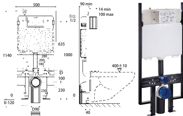
Max working pressure for all cisterns is 5 bar (500Kpa). Test pressure is 20 bar (2000Kpa). Please check wall hung pan set out for correct installation height. Max Weight 250kg.
